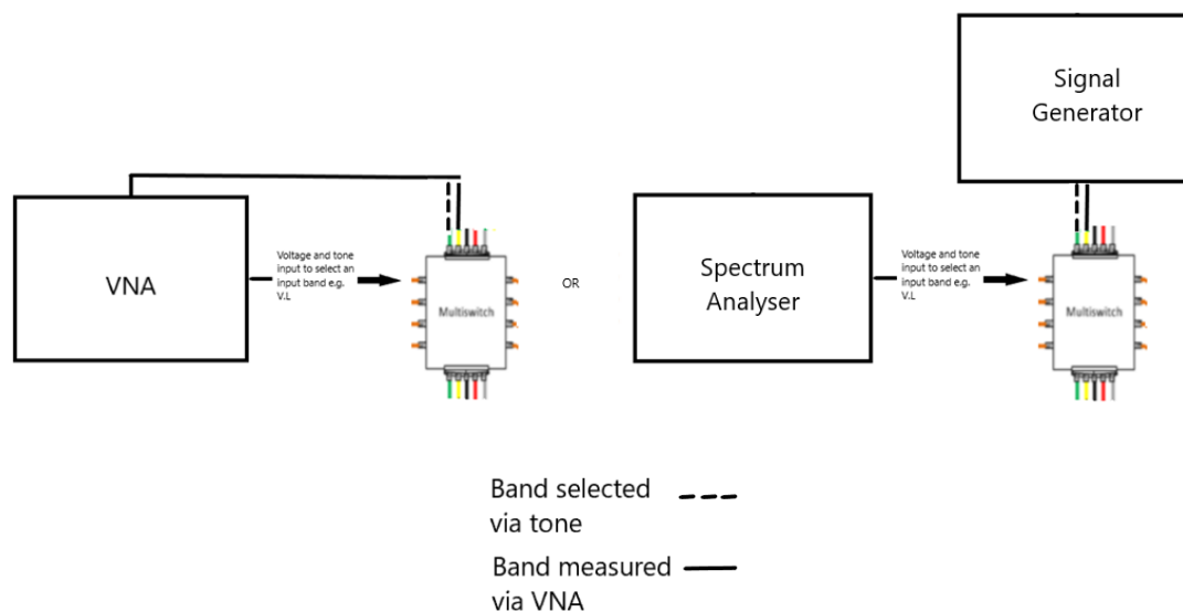
Figure 10 setup for trunk to receiver isolation Step 2
